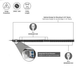
DN-95451 Basic IT PDU, 1-phase 32A, 24 x C13, 4 x C19, 3 m Supply Cable, IEC 60320 C13 A Plug
